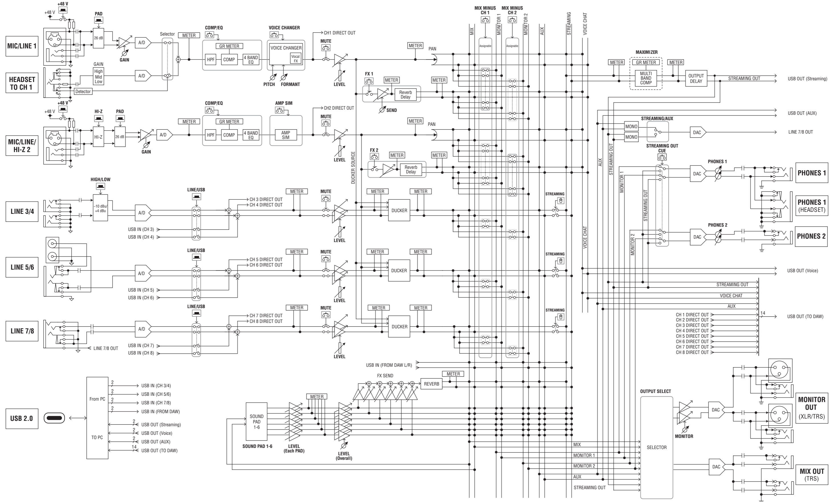
AG08 Mixer Block Diagram (Windows)
